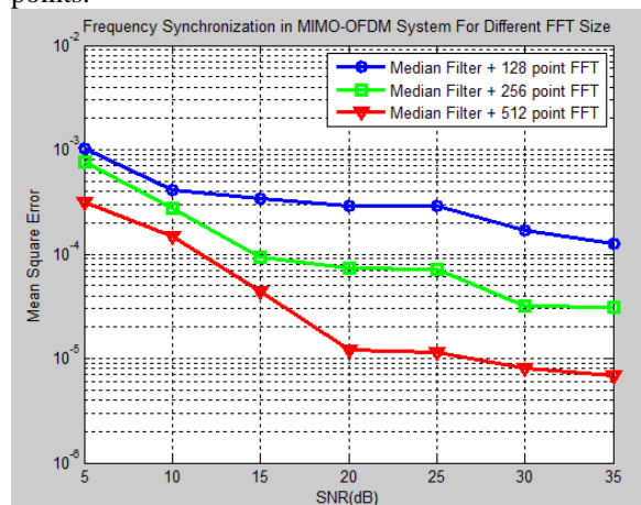
Fig. 5.1 Frequency Synchronization in MIMO-OFDM System with Median Filtering and variable FFT points.
