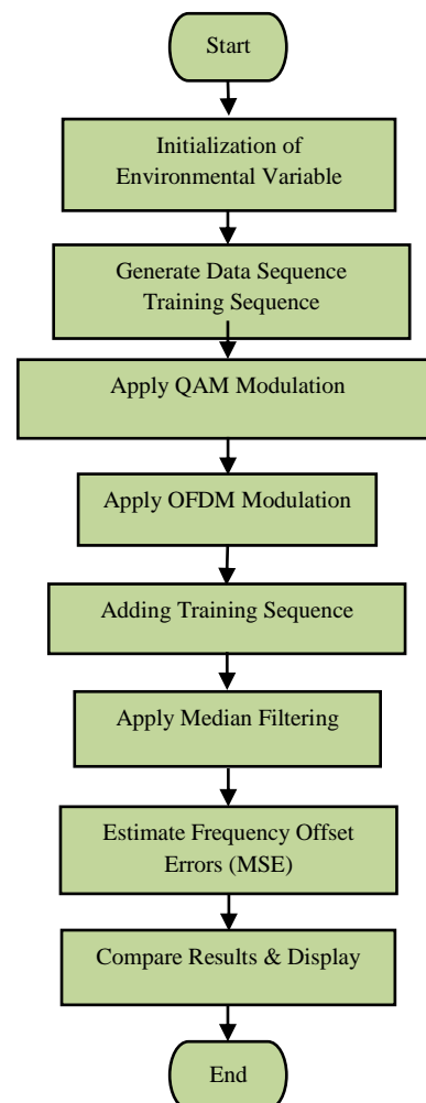
Fig.5.3 Frequency Synchronization in MIMO-OFDM IV. SIMULATION RESULTS
