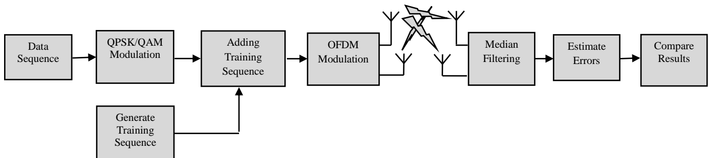
Fig. 3.1 Block Diagram of Time/Freq. Synchronization for MIMO-OFDM
