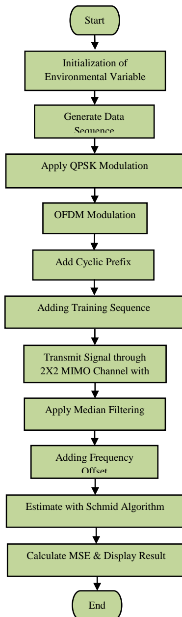
Fig. 3.2 Timing Synchronization in MIMO-OFDM
